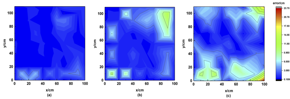
Fig. 10. The positioning results in the location plane for the established VLP system using (a) LSTM-FCN, (b) FCN and (c) SVR algorithm.
