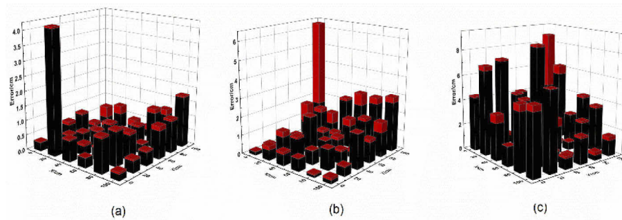
Fig. 7. The error distribution of positioning results in the location plane for the established VLP system using (a) LSTM-FCN, (b) FCN and (c) SVR model.
