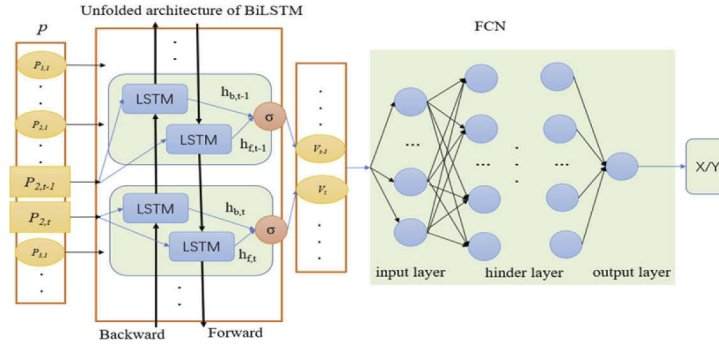
Fig. 1. The structure of LSTM-FCN used in this work for the VLP system.
