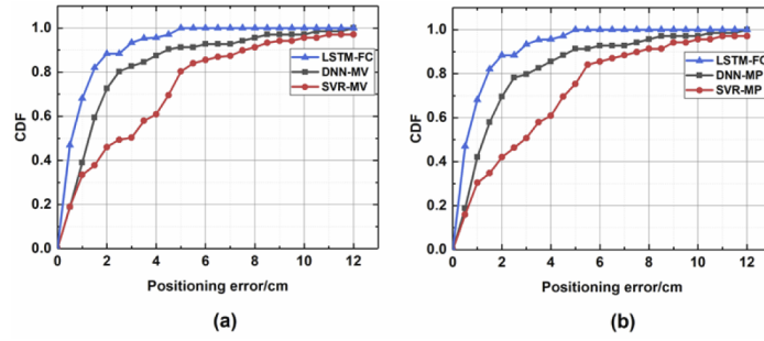
Fig. 9. FCN and SVR with simple denoising methods. (a) mean position value, (b) mean received power.
