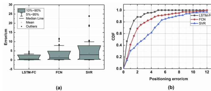
Fig. 8. Positioning accuracy comparison for the established VLP system using different algorithms. (a) BOX, (b) CDF.
