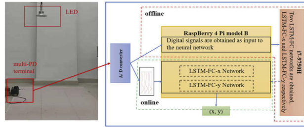
Fig. 2. The structure of the established VLP system using LSTM-FCN.
