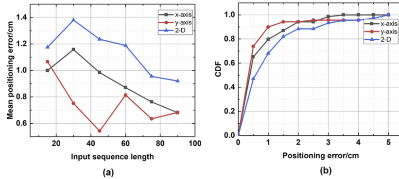
Fig. 6. Error across the different axis. (a) Mean positioning error, (b) CDF.
