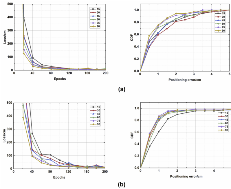
Fig. 5. Training losses and CDF of localization errors for different input sequence length. (a) x -axis, (b) y -axis.
