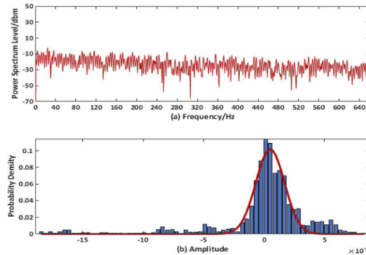
Fig. 4. Noise characteristics of the established VLP system: (a) power spectral density; (b) the distribution characteristics of the amplitude.
